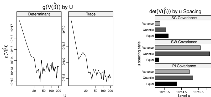
FIG 2.8. Factors of optimal design in the LKC regression: the number of levels U (left) and the spacing mode of the levels u_j (right). The plots show how these factors impact the optimal design criterion g(V[\hat{\beta}]) , for g(M) = \det(M) and g(M) = \text{tr}(M) . Level counts ranging from U = 5 to 200 are considered along with equal, quantile and variance-based spacing. The U plot uses equal spacing and the spacing plot uses U = 50 levels.
