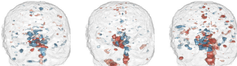
FIG 4.13. Examples of three residual fields from a voxel-wise AR(1) model fit to the FIAC brain data. The scans shown come from the first experimental subject at times 1, 50 and 100. The outer gray layer shows the surface of the brain, while the red and blue show domains with positive and negative residuals, respectively. Light and dark colors represent the data thresholded at the single t -test 95% and 99% thresholds of 1.96 and 2.58.
