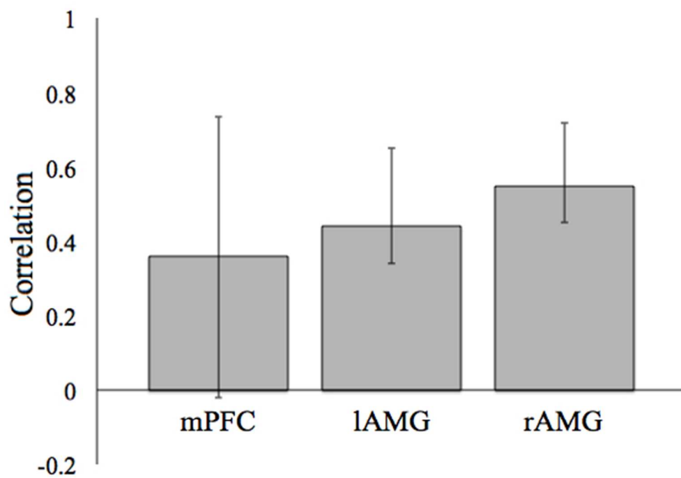
Figure 7. Correlation of activity in mPFC and bilateral amygdala seeds with their respective brain scores show how activity in the three seeds covaries with activity in the entire network. Error bars represent 95% bootstrapped confidence intervals, which indicate no significant differences in the pattern of connectivity between the three seed regions.
