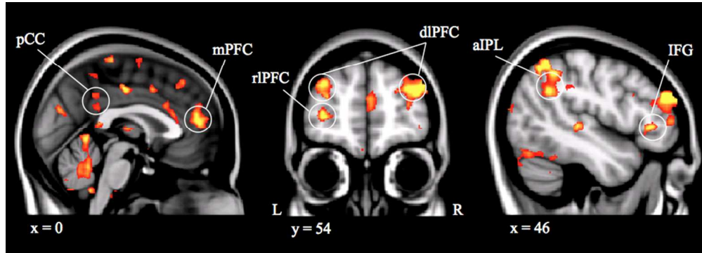
Figure 6. Regions of the distributed functional network in the seed PLS analyses of process simulations.
