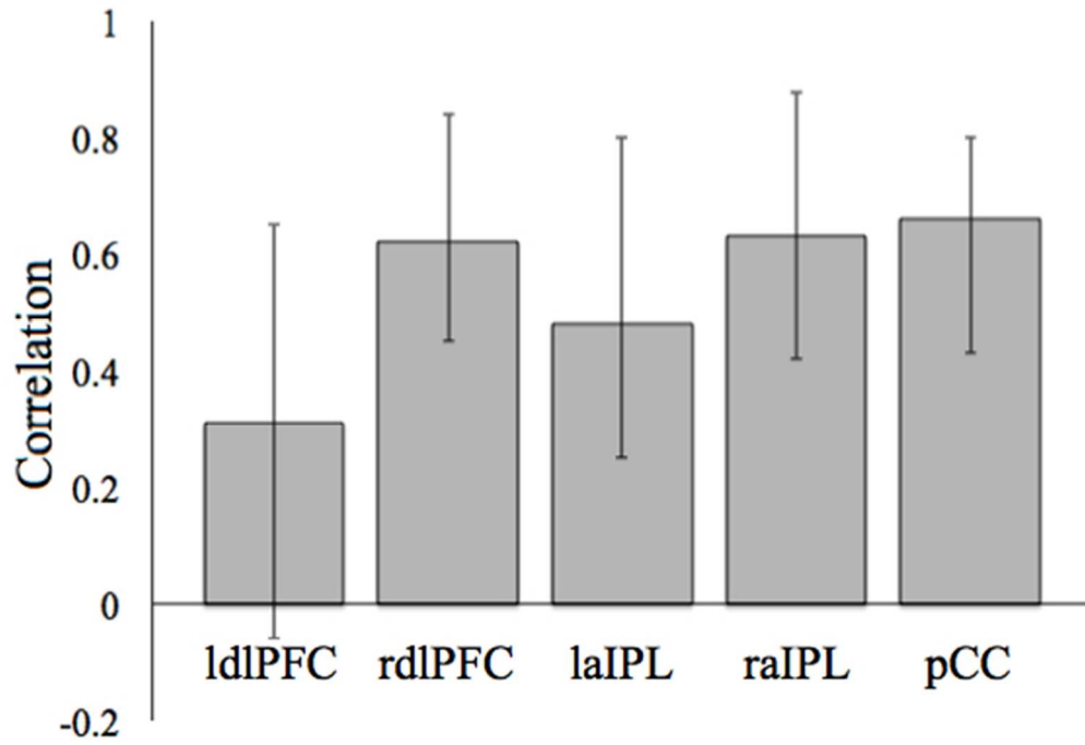
Figure 5. Correlations of activity in bilateral dIPFC, aIPL, and PCC with their respective brain scores show how activity in the five seeds covaries with activity in the entire network. Error bars represent 95% bootstrapped confidence intervals, which indicate no significant differences in the pattern of connectivity between the five seed regions.
