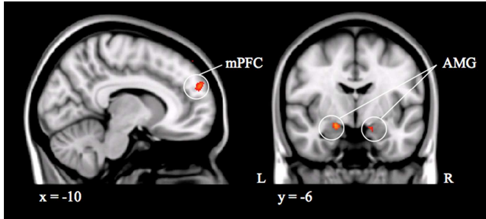
Figure 4. Outcome simulation > Process simulation. Activations in regions of the default network (medial prefrontal cortex) and of the limbic system (bilateral amygdala).
