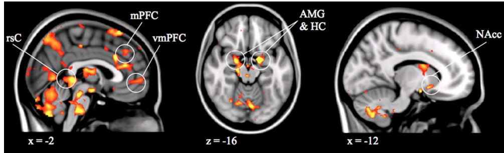
Figure 8. Regions of the distributed functional network in the seed PLS analysis of outcome simulations.
