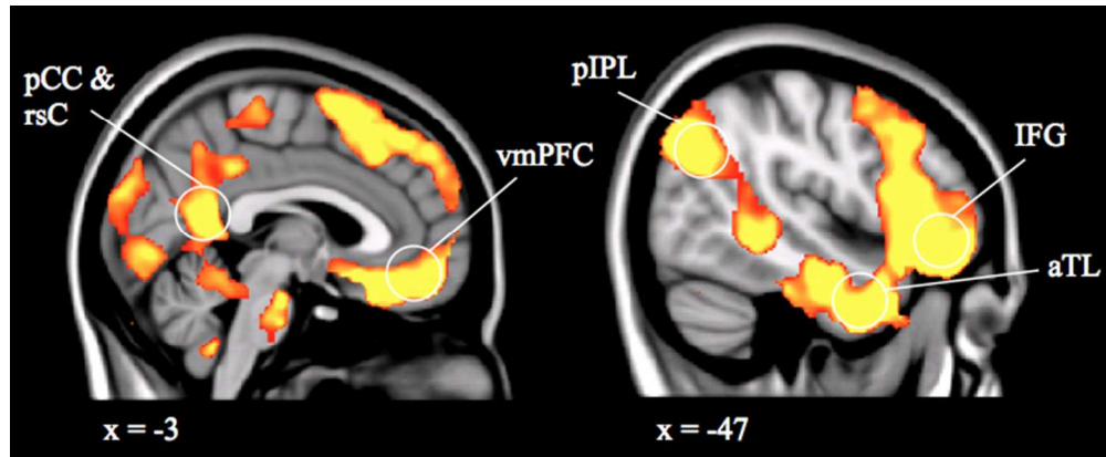
Figure 2. Goal simulations > Odd/Even judgments. Activations in regions of the default network, including posterior cingulate cortex, retrosplenial cortex (rsC), ventromedial prefrontal cortex, posterior inferior parietal lobule, inferior frontal gyrus, and anterior temporal lobe (aTL).
