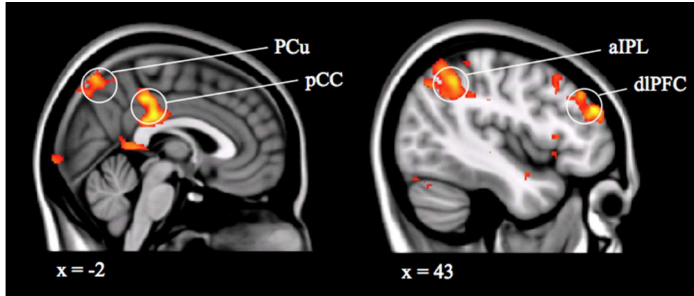
Figure 3. Process simulation > Outcome simulation. Activations in regions of the default network, including posterior cingulate cortex, and regions of the frontoparietal network, such as precuneus, anterior inferior parietal lobule, and dorsolateral prefrontal cortex.
