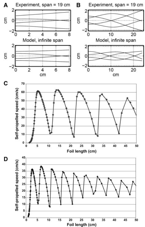
Fig. 2 Results from an inviscid 2D numerical model of propulsion of self-propelled flexible flapping foils (see Alben [2008, 2009b] and Alben et al. 2012 for details of this model) which predicts shape of the foil and the effects of changes in length of the foil on swimming speed. Panels A and B compare experimentally measured and computed midlines of two foils that differ in stiffness, while panels C and D show plots of self-propelled swimming speed versus length for two foils with different stiffnesses. Each point is a separate simulation to calculate the self-propelled swimming speed for that foil. Note the strong resonance peaks that dramatically alter swimming speed as length of the foil changes. Flexural stiffnesses: panel C foil material = 9.9 \times 10^{-4} \text{ Nm}^2 ; panel D foil material = 3.3 \times 10^{-4} \text{ Nm}^2 .
