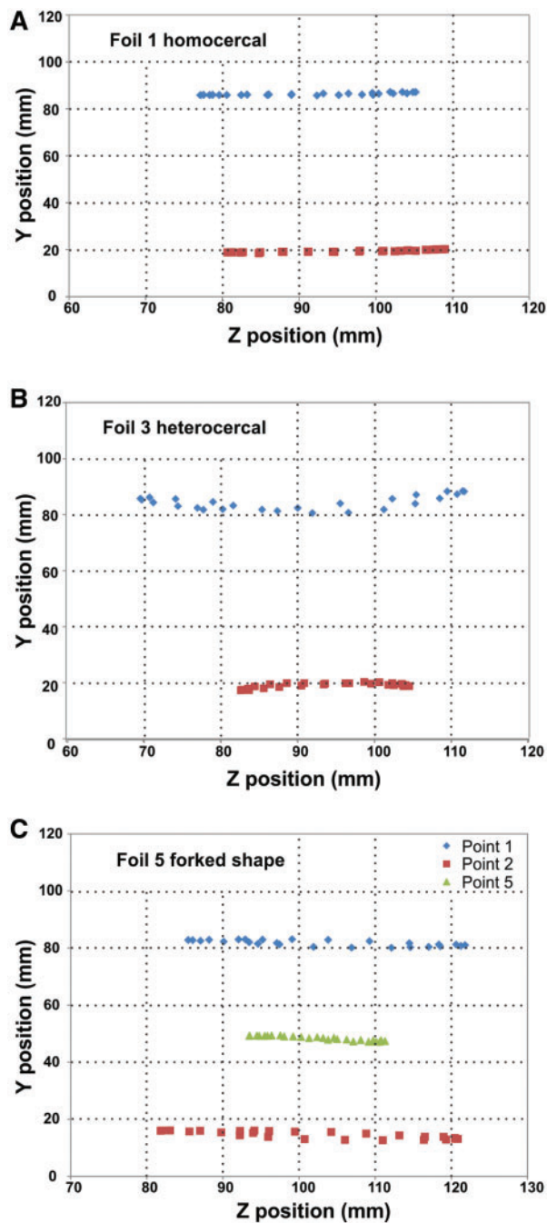
Fig. 9 Kinematics of self-propelled swimming foils (material flexural stiffness = 3.1 \times 10^{-4} \text{ Nm}^2 ). Foil numbers correspond to those shown in Fig. 6. Plots show the YZ plane from posterior view, Fig. 4); point 1 is at the tip of the dorsal trailing edge, point 2 at the tip of the ventral trailing edge, and point 5 is located at the fork of foil 5. Foil 1 has similar excursions (z-axis ranges) of the dorsal and ventral tips of the tail, while the ventral margin of foil 3 undergoes much smaller excursions and both dorsal and ventral tips of this foil move in a curved trajectory, with a concave up and down motion, respectively. Dorsal and ventral tips of foil 5 show greater lateral excursions than do the homologous points on foil 1, while the point in the tail fork moves only half as much as the dorsal and ventral tips.
