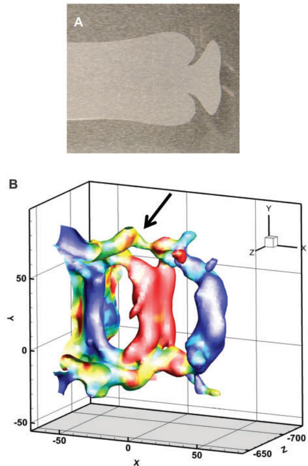
Fig. 7 Visualization of water flow patterns in the wake of the flexible foil shaped like a bluegill tail (panel A) when swimming at its self-propelled speed (material flexural stiffness = 3.1 \times 10^{-4} \text{ Nm}^2 ). This shape (panel A) schematically includes the trailing edges of the dorsal, anal, and caudal fins (see [Drucker and Lauder 2001; Standen and Lauder 2005]). Panel B shows patterns of flow in the wake imaged with volumetric particle image velocimetry (see text for discussion). Vortical connections between the wakes of the caudal and dorsal fins (arrow) are weak when compared to those observed in live fish. Wake vorticity is isosurfaced and then colored by Y vorticity—red is high positive ( 6.5 \text{ s}^{-1} ), blue low ( 1.0 \text{ s}^{-1} ); X, Y, and Z axes delimit the volume visualized, and units are in millimeters. (Reference to color applies to online version, not to printed black and white version.)
