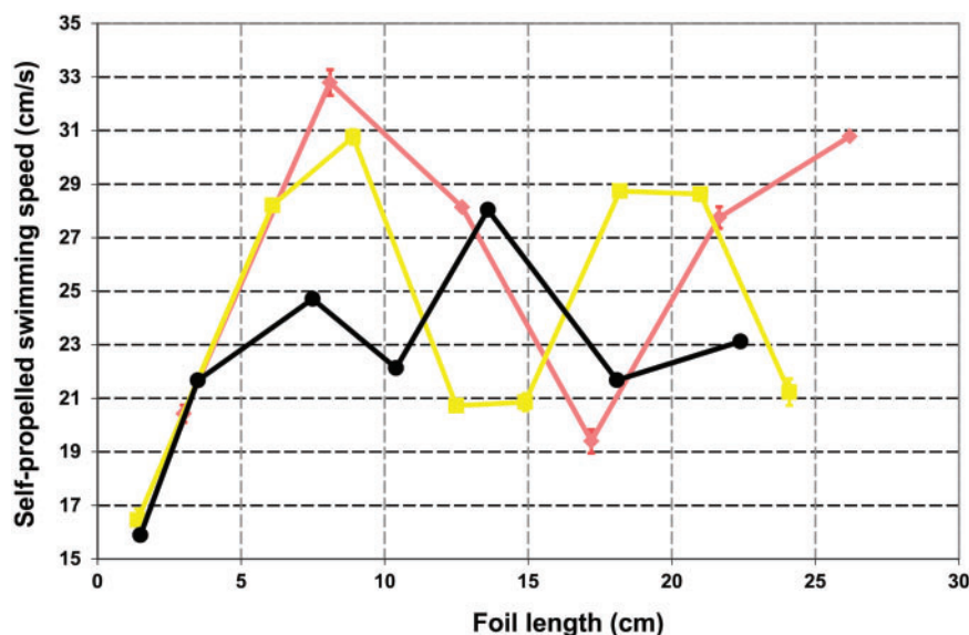
Fig. 1 Experimental data measuring self-propelled swimming speed versus foil length for flexible foils of three different flexural stiffnesses. Foils were actuated with \pm 1.0 cm heave amplitude at the leading edge at a frequency of 2 Hz, with no pitch motion. Error bars of \pm 1 SE are plotted for each point, but some error bars are obscured by the symbols. Note that certain stiffnesses of foils (yellow plot) show multiple peaks in swimming speed as length of the foil changes, and that even relatively small changes in length can have substantial effects on swimming speed. Foil flexural stiffnesses: coral color = 4.9 \times 10^{-3} Nm 2 ; yellow = 9.9 \times 10^{-4} Nm 2 ; black = 0.32 \times 10^{-4} Nm 2 . (Reference to color applies to online version, not to printed black and white version.)
