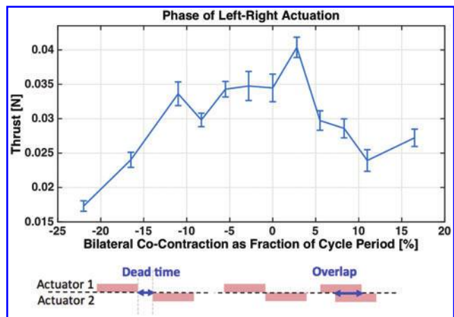
FIG. 6. Measurement of thrust as a function of co-contraction phasing between the right and left sides in undulatory swimming of a soft robotic fish-like model at 0.55 Hz while exposed to continuous water flow speeds of 5.3 cm/s. Each thrust data point represents a mean over a trial length of 30,000 samples over a total cumulative duration of 120 s from five trials. (A) Contraction phasing for actuation left-right side actuation is represented as percent periodic time for experiments with a latency of -22\% cycle period or -400 ms, and -300 ms, -200 ms, -150 ms, -100 ms, -50 ms, respectively, with such delay designated as “dead time”. Overlapping actuation between the left and right sides is shown as a positive value up to 17% of cycle period, while the extent of nonoverlapping actuation is presented as a negative latency. (B) Schematically the pattern of bilateral actuation corresponding to the respective regions in the graph above. Color images available online at www.liebertpub.com/soro
